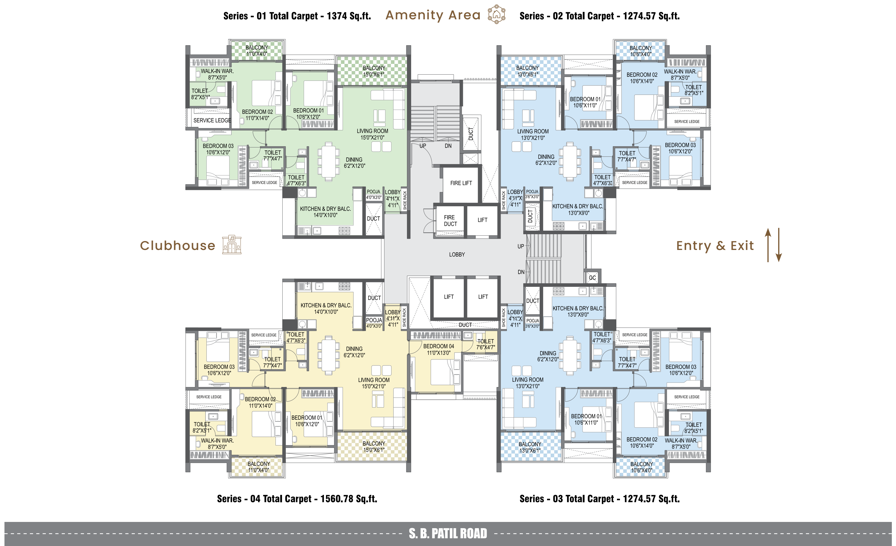
WING-D | TYPICAL FLOOR PLAN
